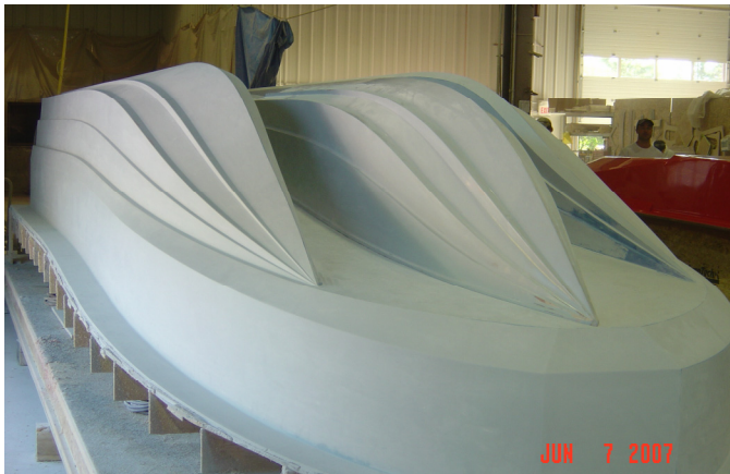
The patented Reflex tri-hull in 28 ft tooling form.
